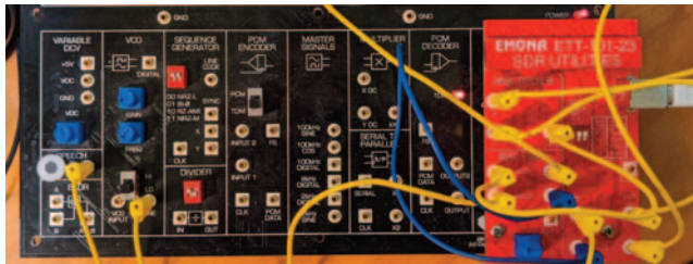
- SDR Experiment patching on the hardware
