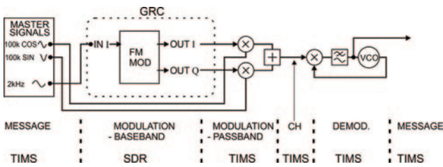
- SDR Experiment block diagram
