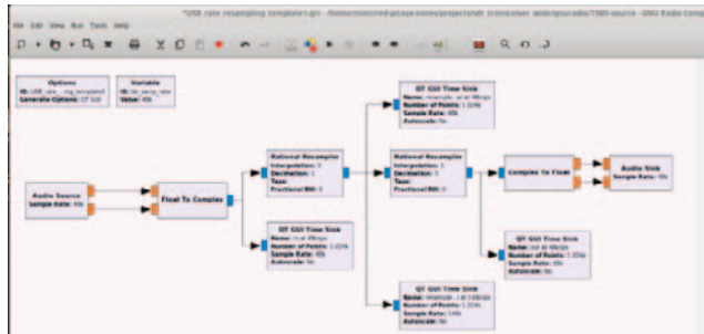
- Launching GNURadio
