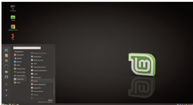
- Launching LINUX
